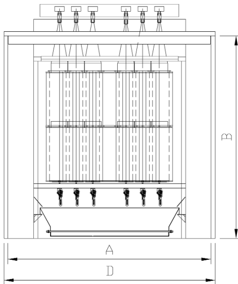
FRONT ELEVATION VIEW SHOWN WITH OPTIONAL FLUIDIZING HOPPER
