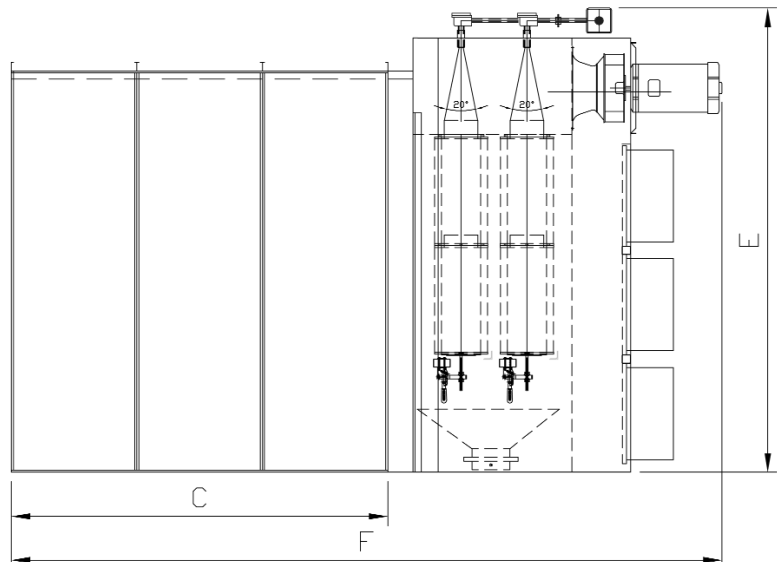
SIDE ELEVATION VIEW SHOWN WITH OPTIONAL FLUIDIZING HOPPER
