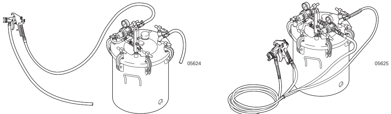
Figure 4: Single regulated pressure pot (left) and dual regulated pressure pot (right).
