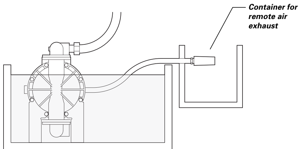
Figure 9: Submersion feed system.
