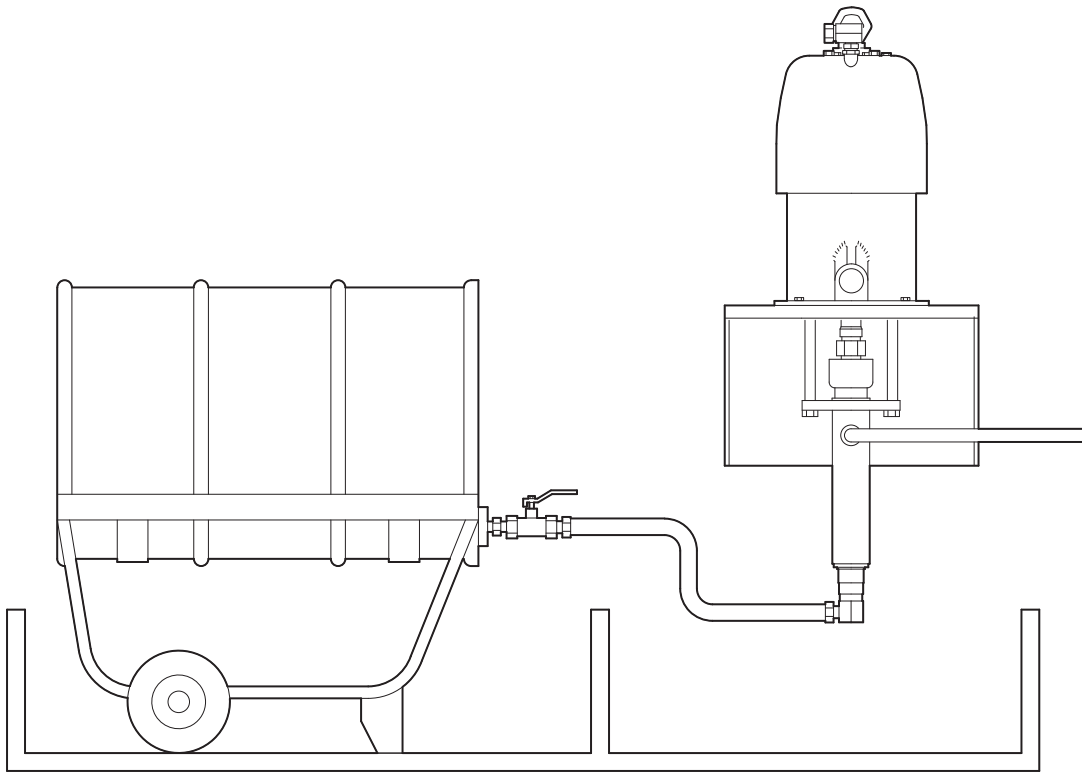
Figure 8: Gravity feed system inside containment barrier.
