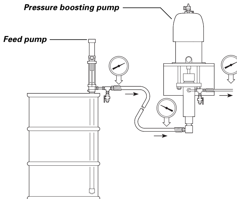
Figure 6: A shorter suction hose, a larger diameter suction hose, or a feed pump (illustrated here) can help increase fluid pressure at the pump inlet.
