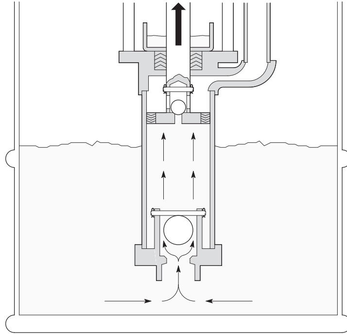
Figure 5: A positive supply of fluid (positive fluid pressure) is required to load a reciprocating piston pump.
