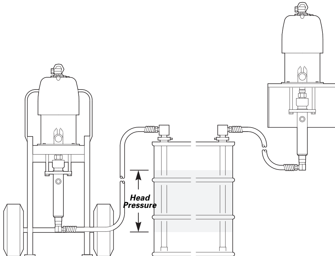
Figure 7: Two types of siphon feed systems: siphon feed with benefit of head pressure (left) standard (right).
