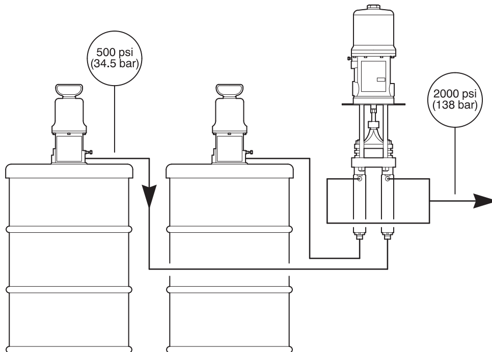
Figure 13: Illustration of 25 percent pressure feed rule, which says that the feed supply pressure should not exceed 25 percent of the output fluid pressure of the piston pump being fed.
