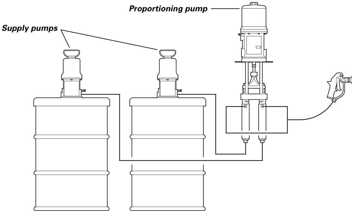
Figure 12: Typical pressure feed system: 5:1 ratio pump feeding a proportioner.
