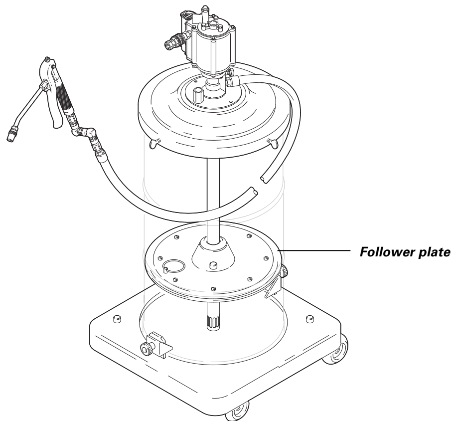
Figure 11: Follower plates are used in immersion feed systems with highly viscous materials.
