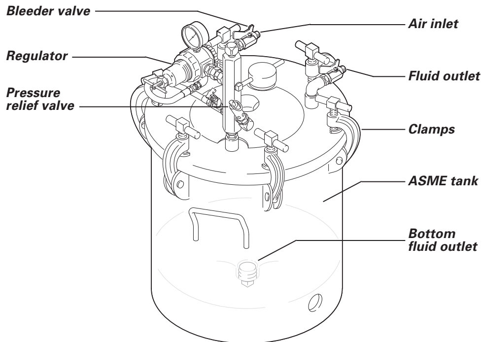
Figure 3: A pressure pot and its key components.
