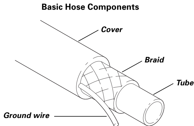
Figure 19: Four main components of a basic hose.
