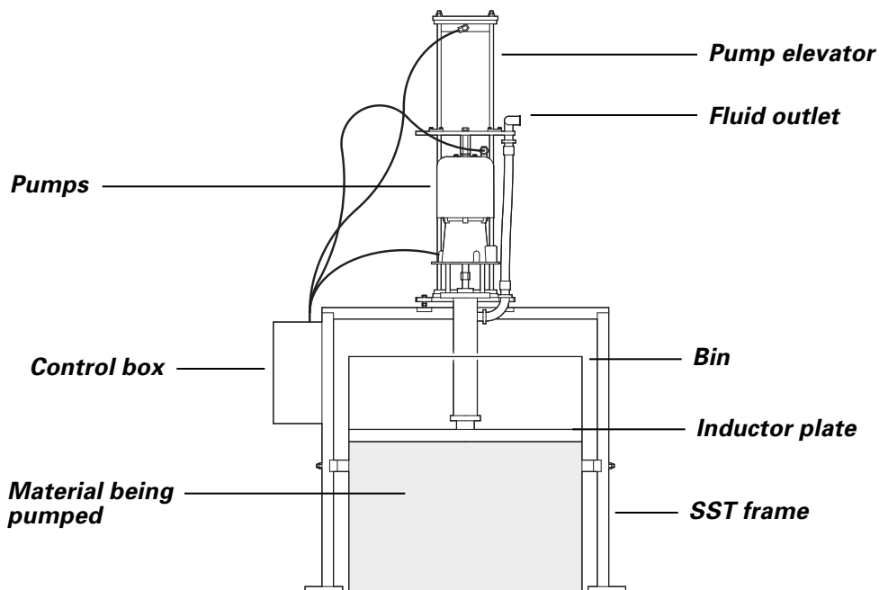
Figure 17: An example of a bulk unloading system.
