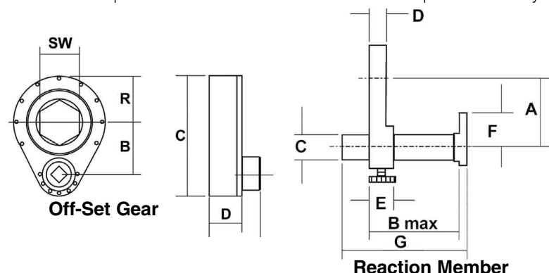
Reaction Member
