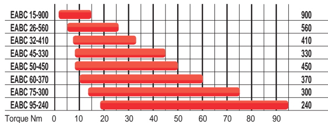
Angle head tools (EABCCom) ROTATIONAL SPEED rpm
