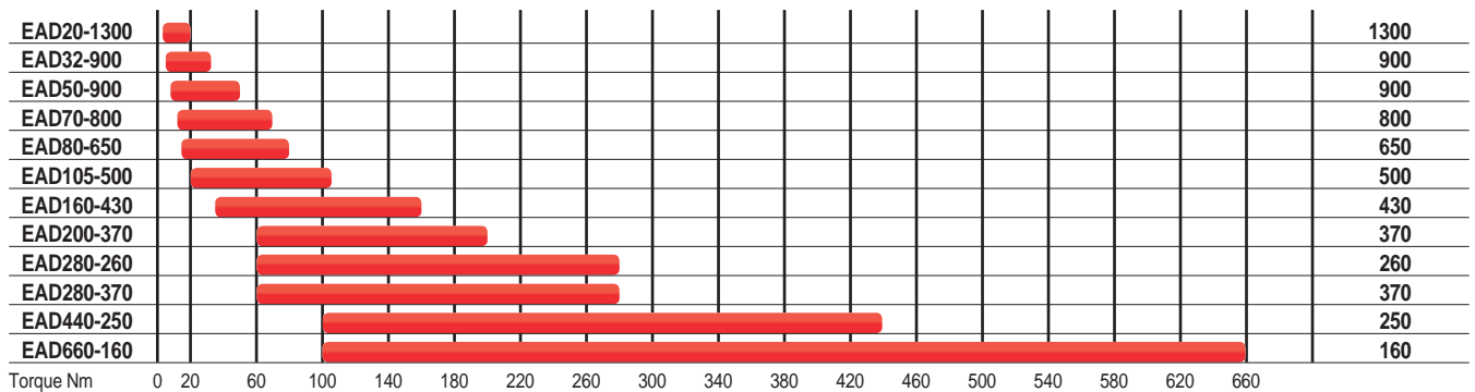
Angle head tools (EAD) - Widest Torque Ratio ( T_{max}/T_{rpm} ) 5.2 ROTATIONAL SPEED rpm
