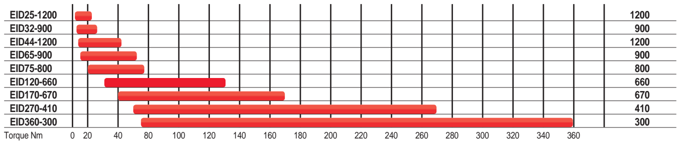
Angle head tools (EABCCom) ROTATIONAL SPEED rpm
