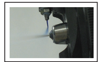
The Binks vinyl ester system features the highly acclaimed Binks Century HVLP vinyl ester spray gun.
